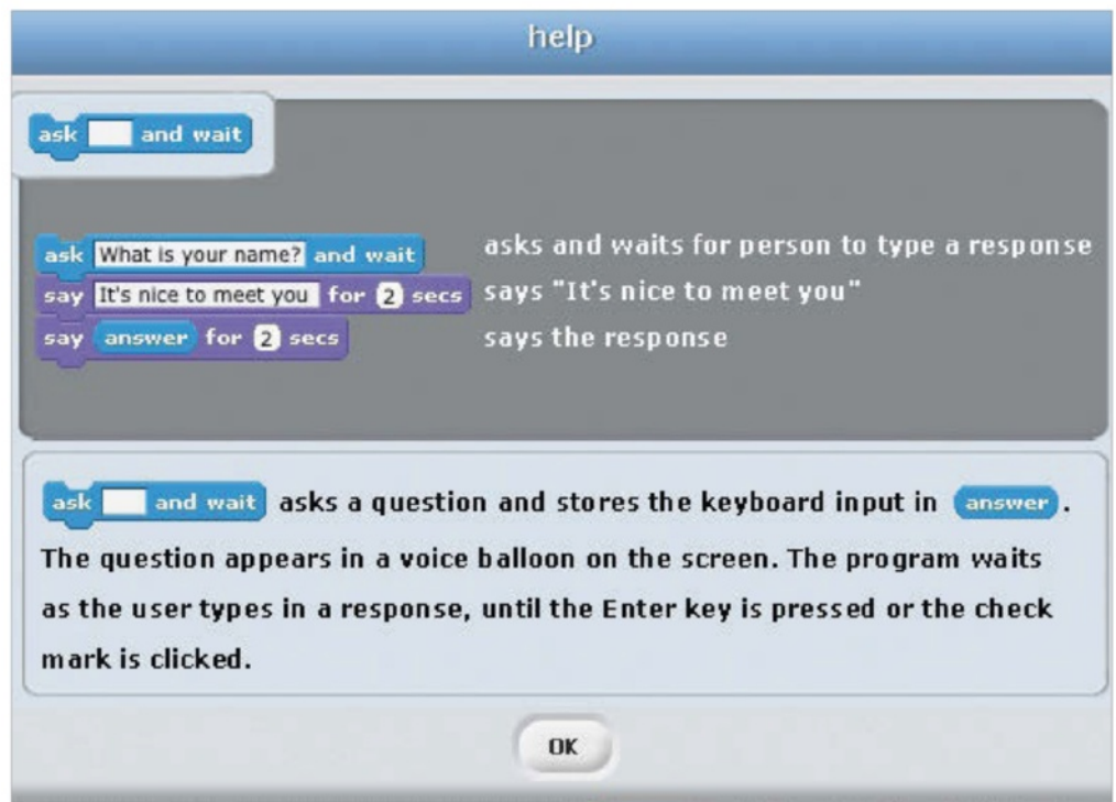
■ Fig 4: Block Help Window – Example of the help window associated with an 'ask and wait' block
